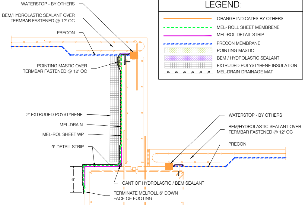
2 WATERPROOFING DETAIL @ STEP DOWN W2.03 3"=1'-0" Rev: 8/S20.01
