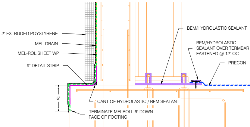
3 CAISSON TERMINATION DETAIL W2.03 3"=1'-0" Rev: 8/S20.01
